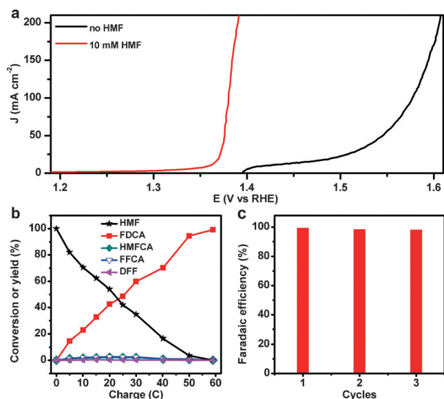
Figure 2. a) LSV curves of Ni 2 P NPA/NF at a scan rate of 2 mV s -1 in 1.0 M KOH with and without 10 mM HMF. b) Conversion and yield (%) changes of HMF and its oxidation products during the electrochemical oxidation of HMF at 1.423 V vs. RHE in 1.0 M KOH with 10 mM HMF. c) Faradaic efficiencies of Ni 2 P NPA/NF for FDCA production under three successive electrolysis cycles.
